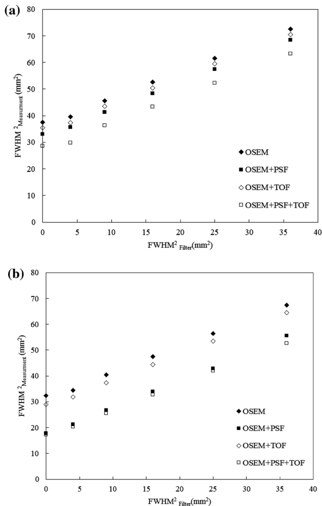
Fig. 2 Measured FWHM for capillary tubes embedded in the air as a function of post-smoothing Gaussian filter for different reconstruction protocols; a it \times sub = 32, b it \times sub = 54
